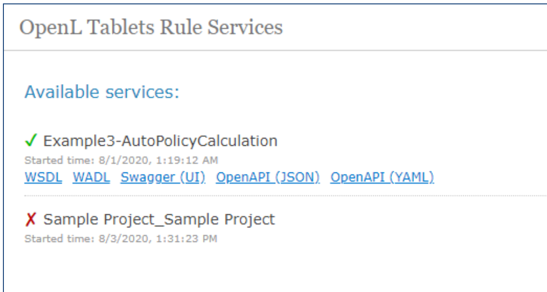
Figure 6: OpenL Tablets Rule Services main page and the project deployed on it
